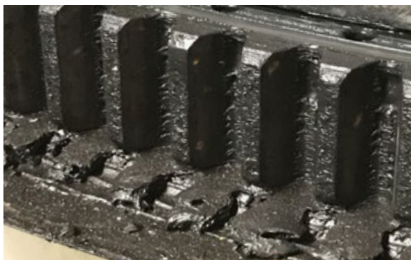
Cleaning of yaw adjustment
